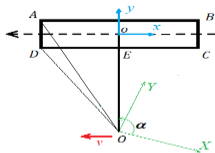
Fig. 3 Geometry and kinematics of the roto translatory movement of a rectangular body in the plan.
