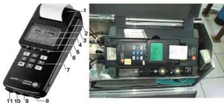
Figure 2. Control unit: 1 - printer; 2 - touch-pen; 3 - system information bar; 4 - display of measured values; 5 - bar for operation information; 6 - function operation keys; 7 - keyboard; 8 - pressure probe connection; 9 - sample connection; 10 - analysis unit connection; 11 - serial interface.
