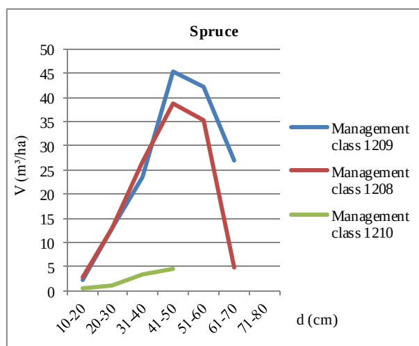
Graph 4. The distribution of the volume of the spruce trees for different management classes in relation to DBH.
